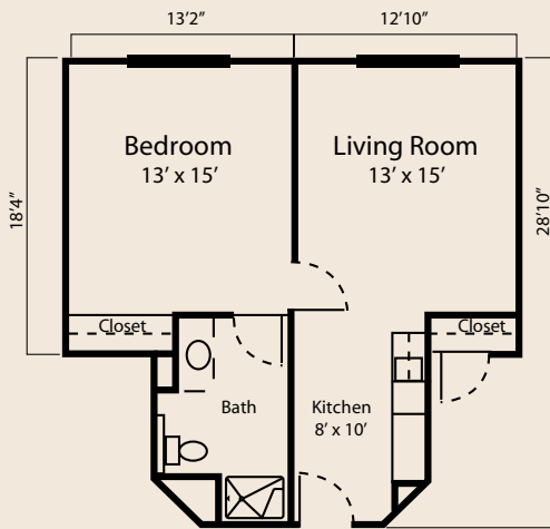
One-Bedroom
